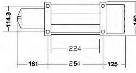
Bolting Pattern
